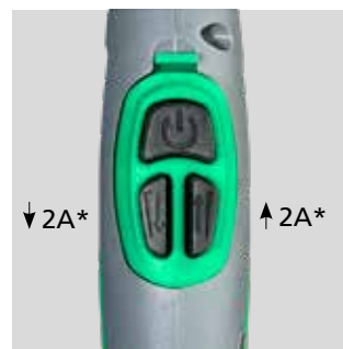
Up/Down module with 3-function key for adjustment of welding current. The welding current is increased / reduced with 2 amps. Long press for constant increase / decrease. 80300064
