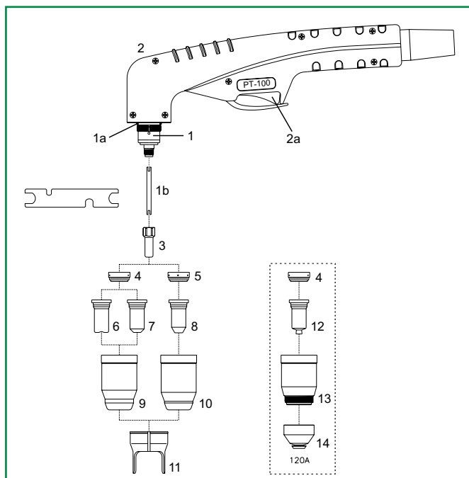
Wearing part box for Zeta 100.
