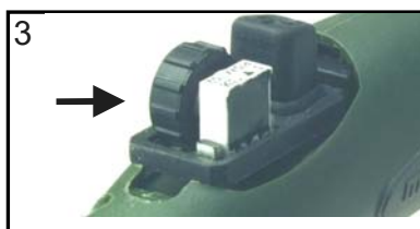
Up/Down modul med 3-knap-tast til justering af svejsestrøm Up/Down module with 3-function key for adjustment of welding current 80300064 (released after Oct. 2012)
